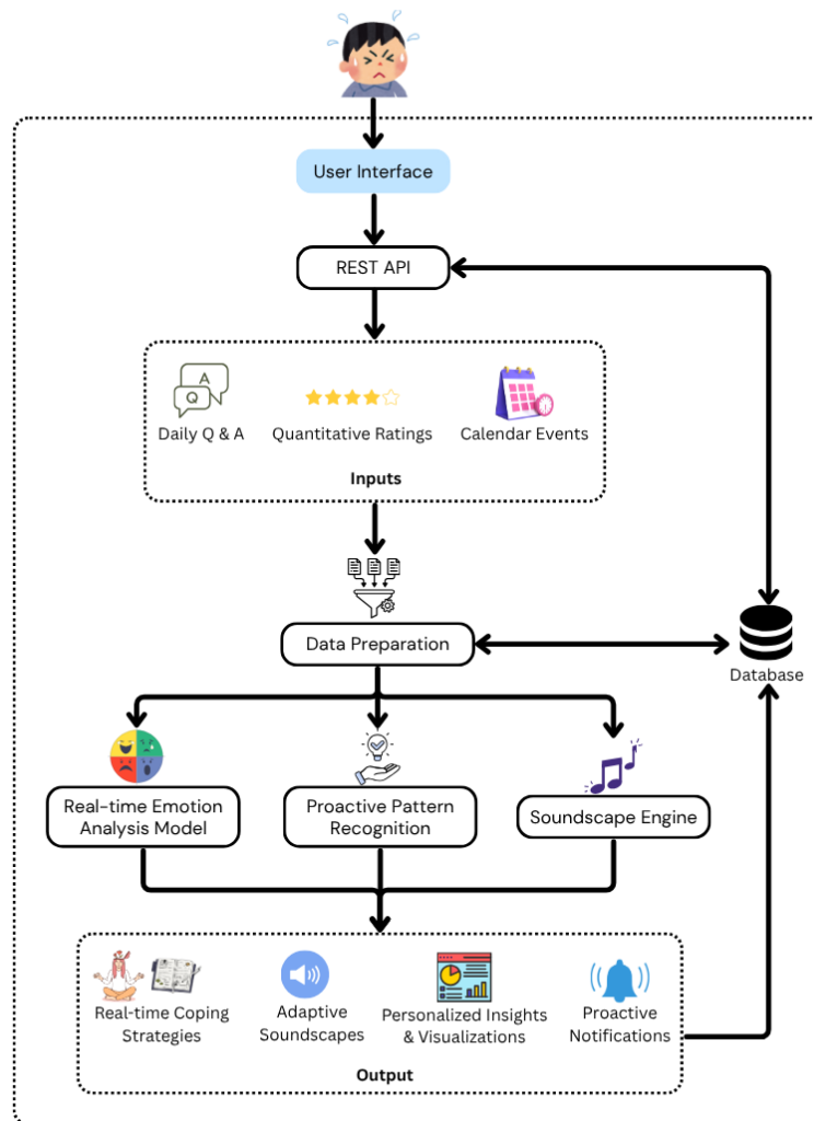
Figure 1 System Architecture
